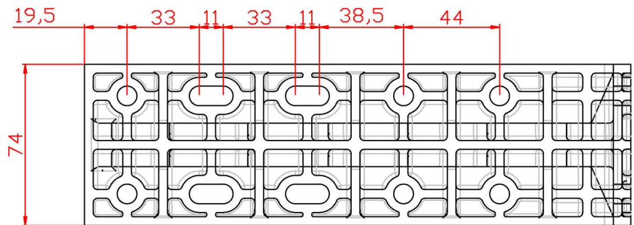
SLB - Thermokonsole TKP 250/300 L
